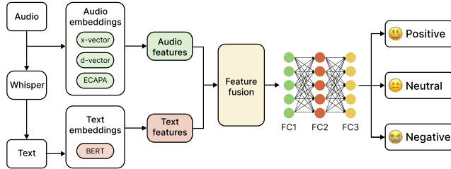
Figure 4: The workflow of our speech emotion recognition
